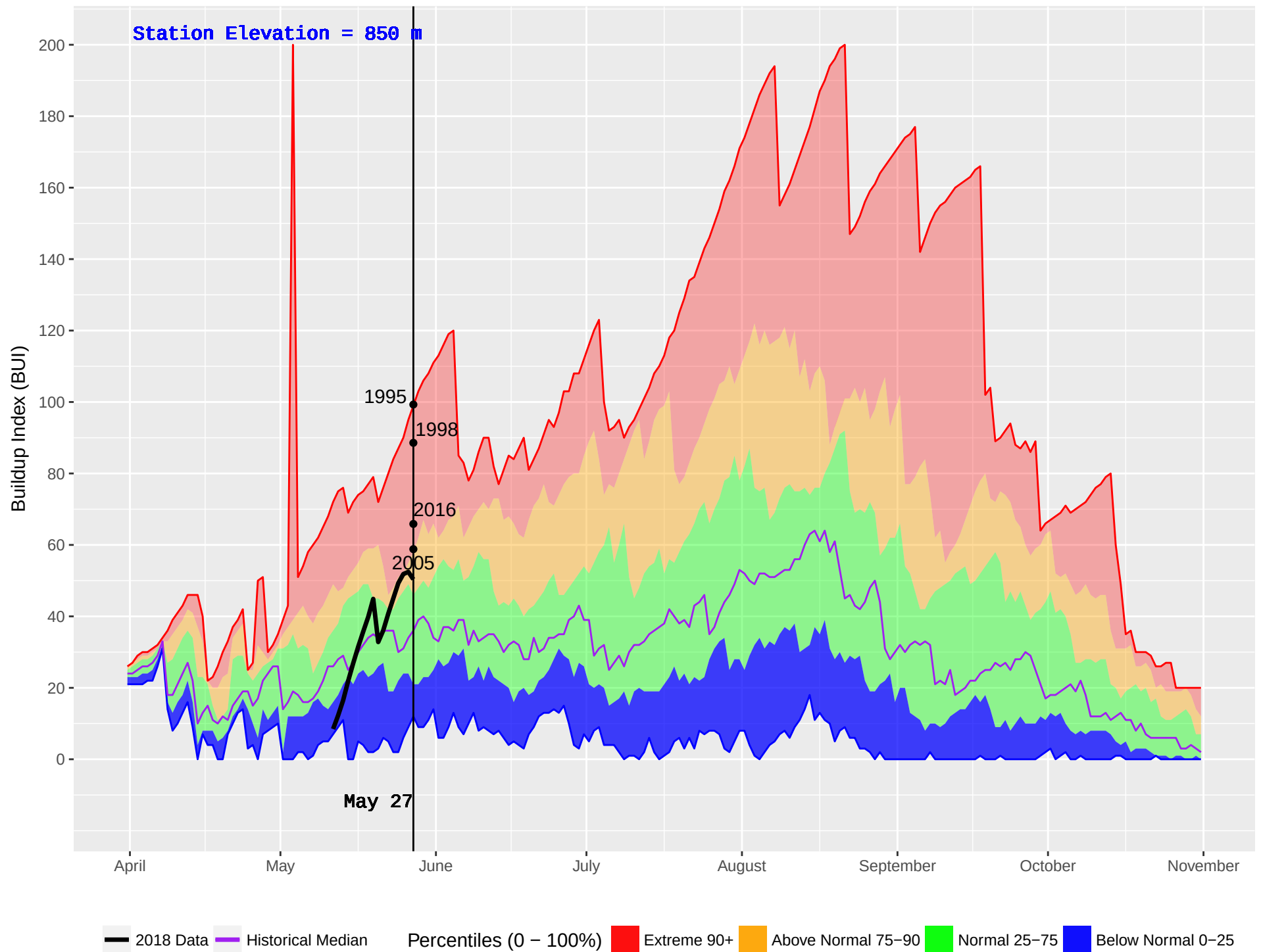
NORTH CHILCO (159) : Historical (1972–2016) and Current (2018) Noon Buildup Index (BUI)
