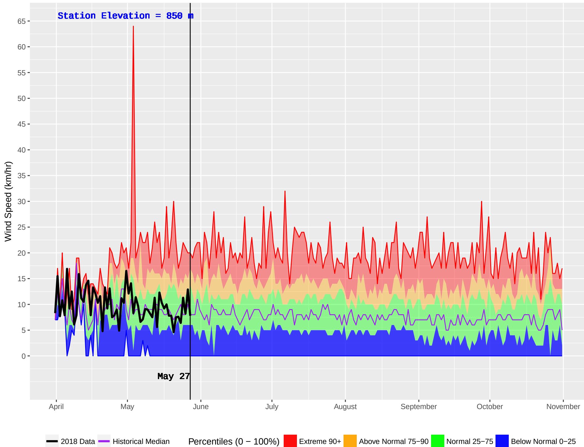
NORTH CHILCO (159) : Historical (1972–2016) and Current (2018) Noon Wind Speed
