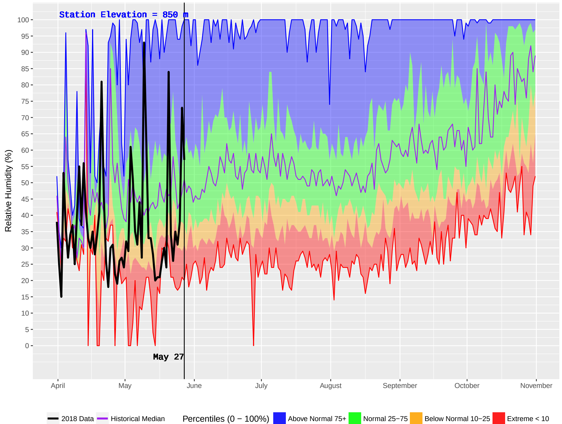
NORTH CHILCO (159) : Historical (1972–2016) and Current (2018) Noon Relative Humidity
