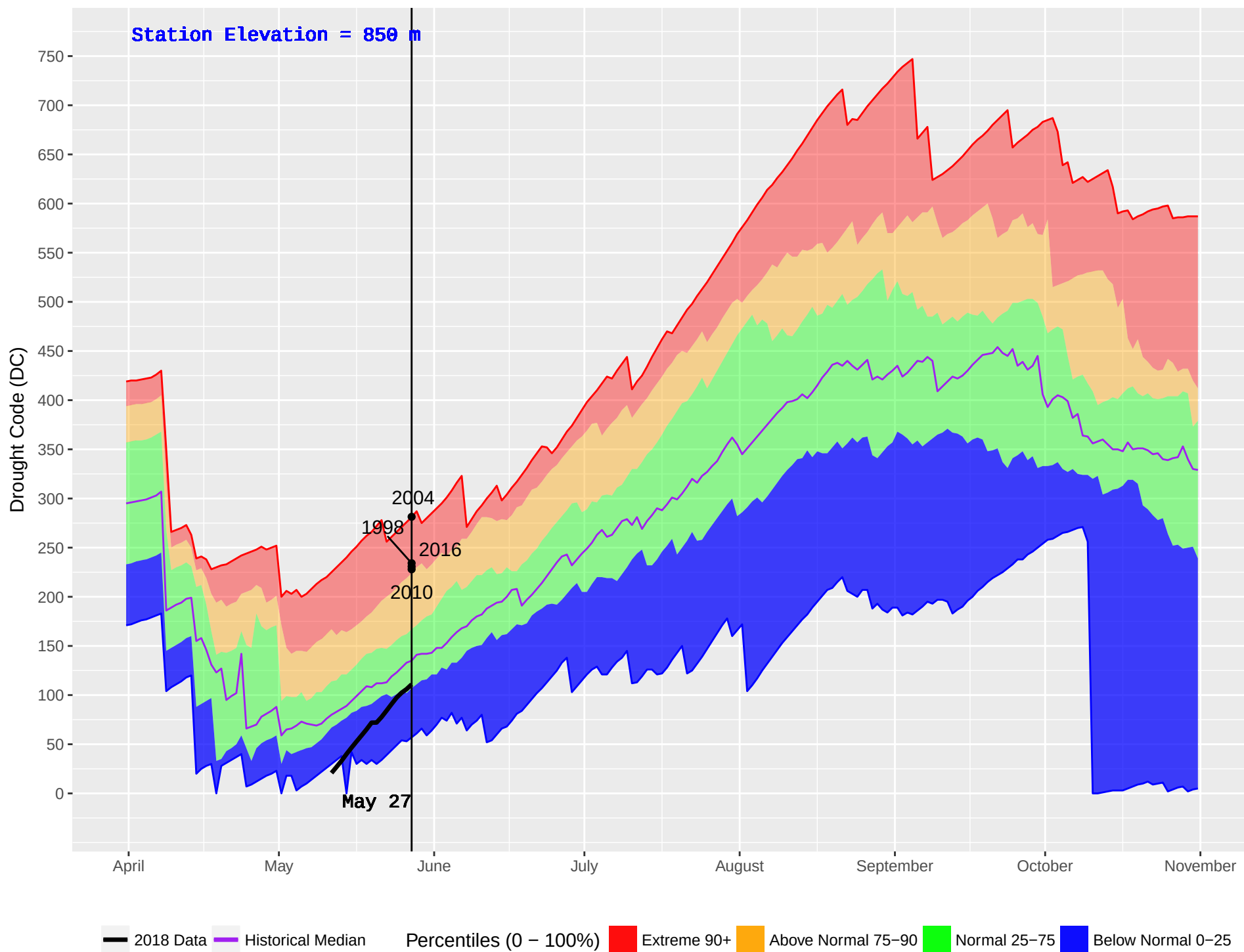
NORTH CHILCO (159) : Historical (1972–2016) and Current (2018) Noon Drought Code (DC)
